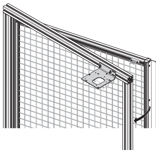
Schmersal AZM 161...
