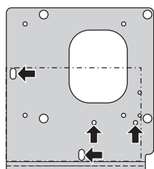
Schmersal AZM 161...
