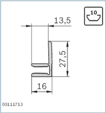
Clamping profile 2S, 8 mm slot
