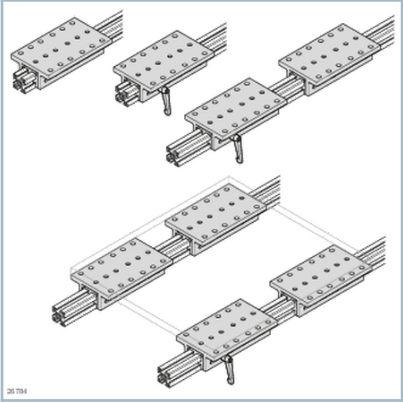
EcoSlide 45x60x160 sliding carriage with clamping holder
