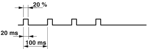
Fig. 10 Pulse generator: number of pulses = 4, duty factor = 20%, pulse width = 20 ms, period = 100 ms
