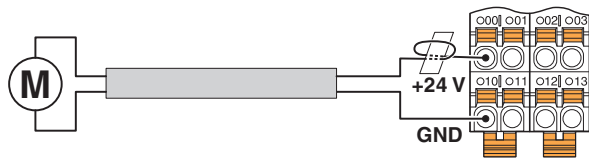
Fig. 4 Connection when a ferrite clamp is used
