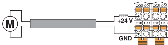
Fig. 5 Connection when chokes are used
