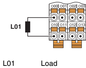
Fig. 3 Connection example
