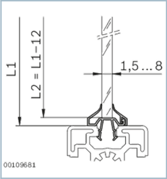
Protective pane profile, PVC
