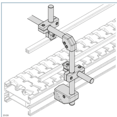
Holder for height-adjustable guides
