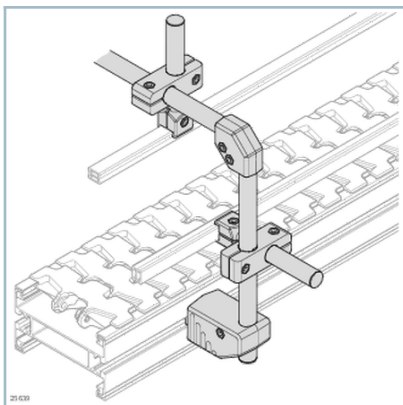
Clamping holder, clamping head
