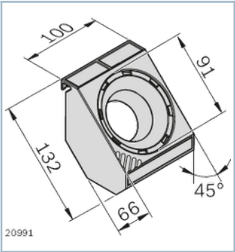
Bucket-tray D91-32 (with base)
