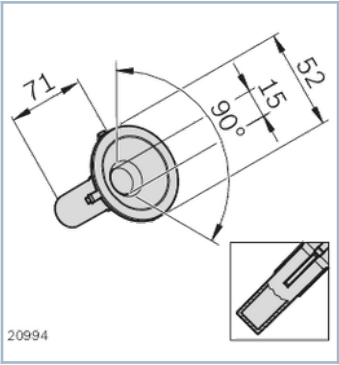
Tool holder D91
