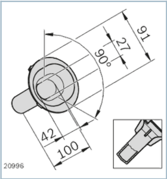
Bucket-tray D91 Oval53 L100 (with base)
