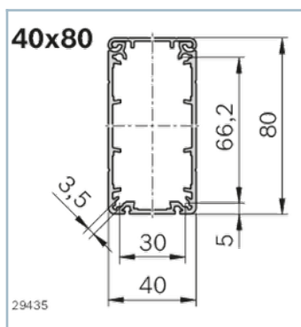
Cable duct with AL cover plate 80x40
