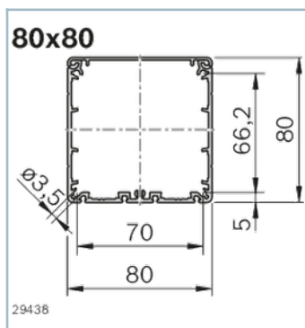
Cable duct with AL cover plate 80x80
