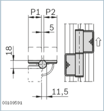
Hinge, removable
