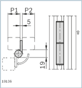
Hinge, removable
