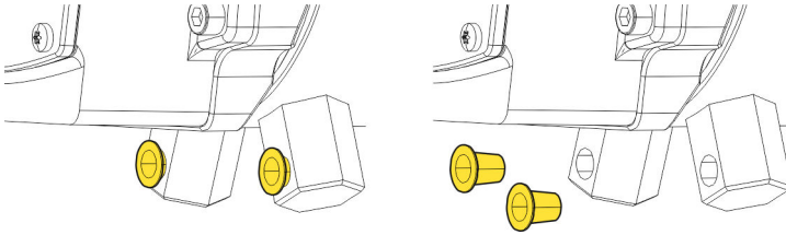
Fig. 30: Protective plug MS2N07, MS2N10 water cooling
