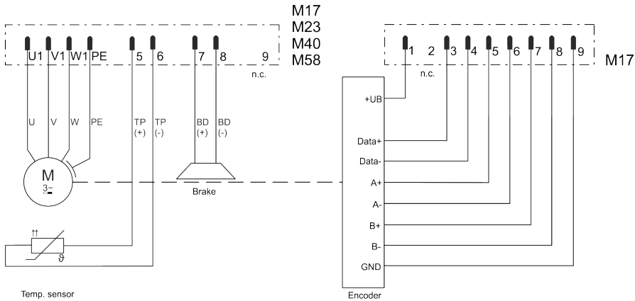
Fig. 13: Double cable connection, analog encoder “A/B”, optional brake
