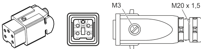
Fig. 23: RLS0782 fan connector individual components
