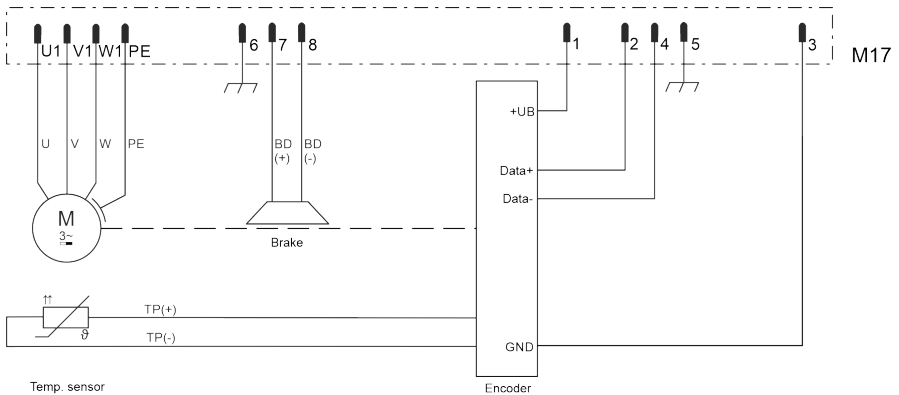
Fig. 11: M17 Single cable connection, digital encoder “C / D / H / J / M”, optional brake
