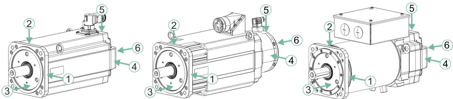
Fig. 33: Vibration load on measuring points
