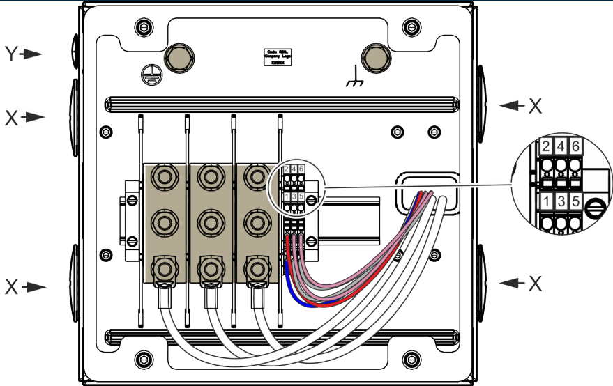
Pin assignment, terminal boxes “E” , power
