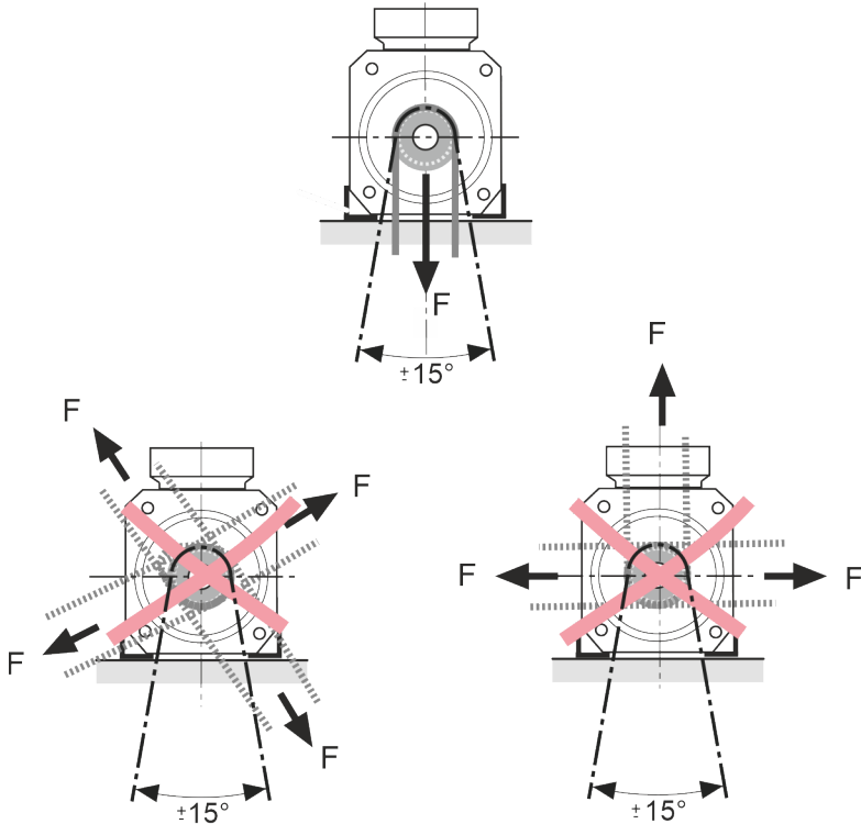
Fig. 9: Force direction at foot mounting
