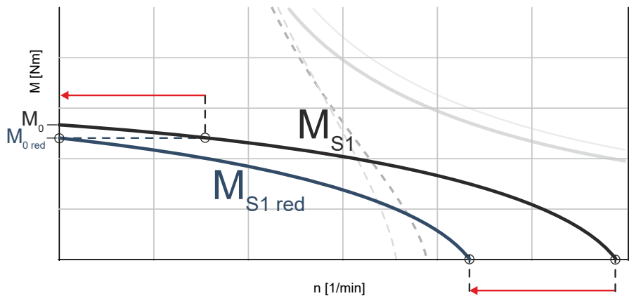
Fig. 34: Determine S1-characteristic curve M_{S1 \text{ red}} with derating factor f_{rH}
