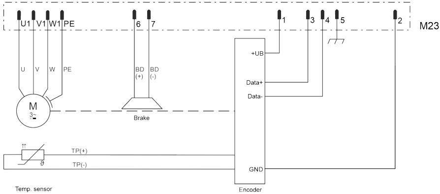
Fig. 12: M23 Single cable connection, digital encoder “C/D/H/J/M”, optional brake
