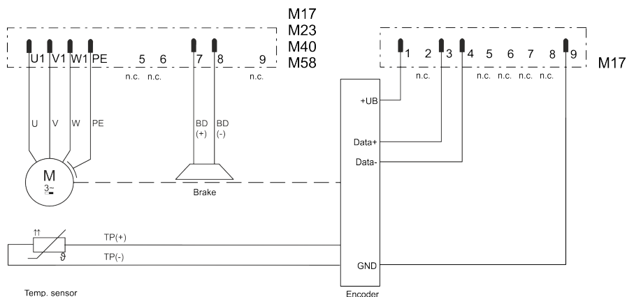
Fig. 14: Double cable connection, digital encoder "C/D/H/J/M", optional brake
