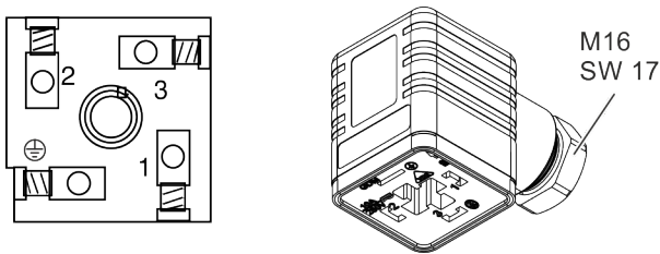
Fig. 21: RLS fan connector individual components
