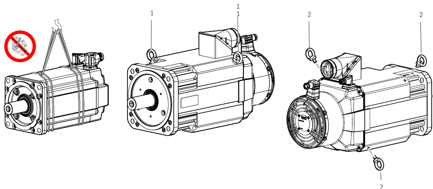
Fig. 8: Lifting and transporting motors
