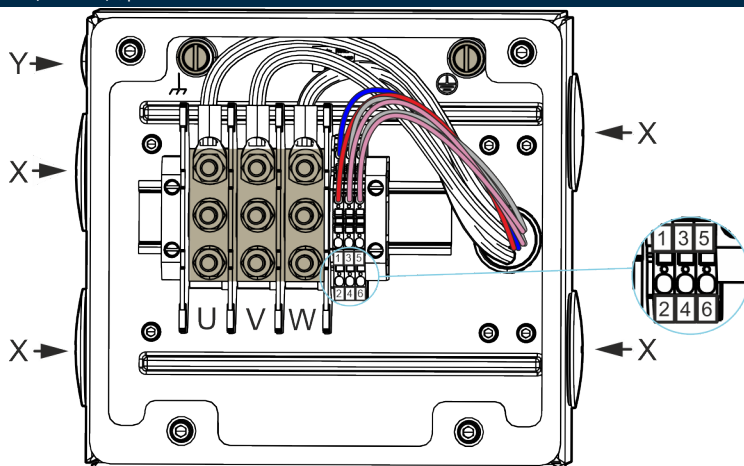
Pin assignment, terminal box "C (MS2N13)", power
