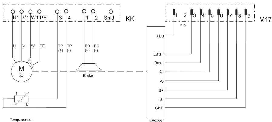
Fig. 15: Double cable connection terminal boxes, analog encoder "A/B", optional brake
